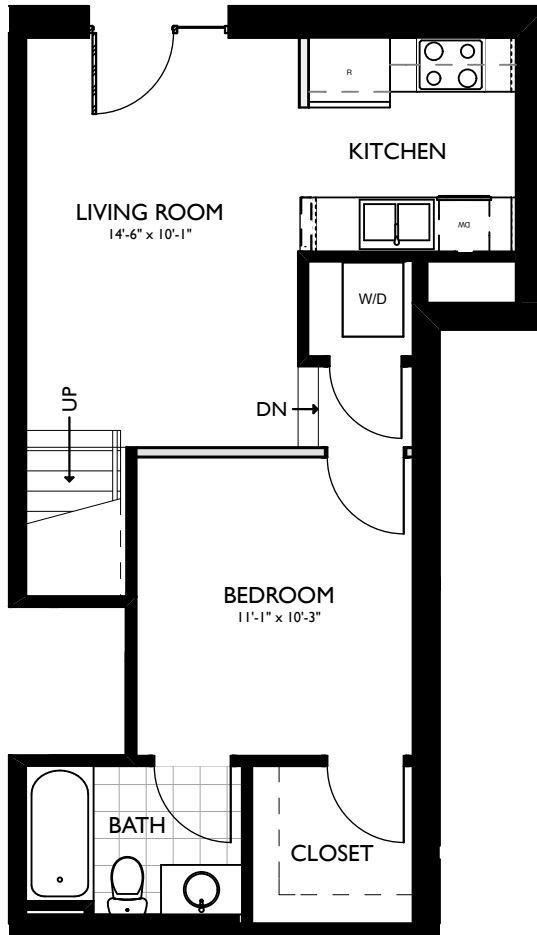
LOWER FLOOR
